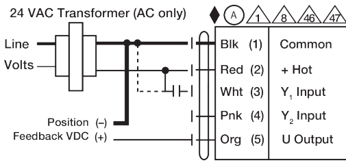
PWM Control
